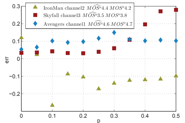
Fig. 3: Prediction error of optimal target MOS across percentiles for three videos streamed over three channels
